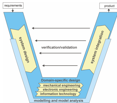
Figure 10: Design process of the VDI-Guideline 2206
