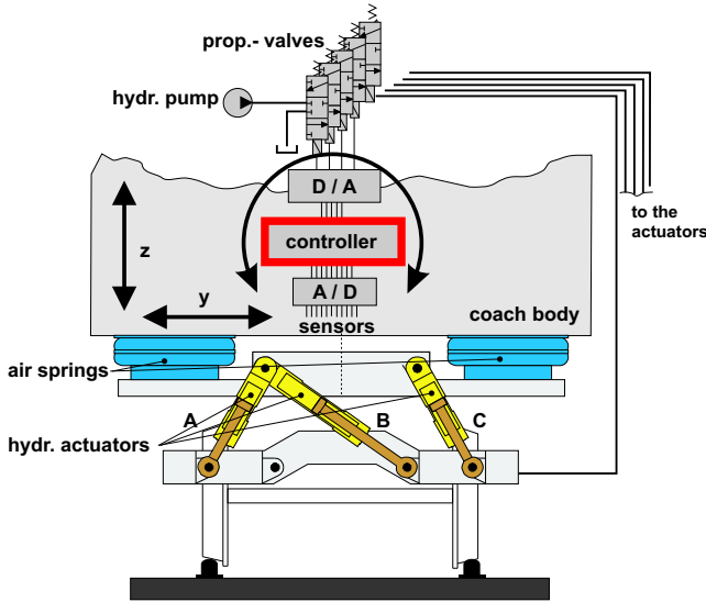
Figure 1: Scheme of the suspension/tilt module
