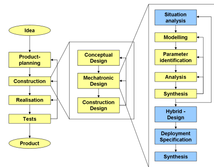
Figure 11: Extended Design process of feedback controller development
