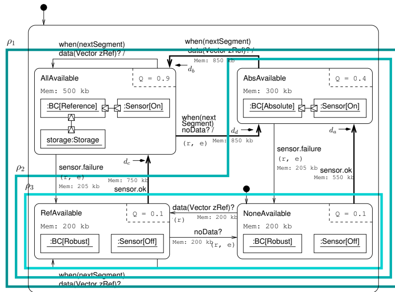
Figure 7: Result of the synthesis algorithm
