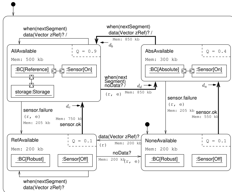
Figure 5: Monitor behavior with annotated resource requirements, quality and transition types
