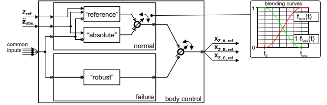
Figure 2: Fading between different control modes
