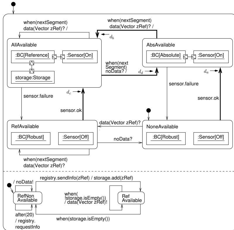
Figure 4: Behavior of the monitor component with modular reconfiguration of the subcomponents
