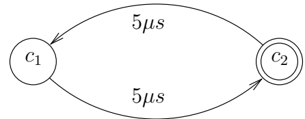
Figure 6: A simple example for profiles and their reachability graph
