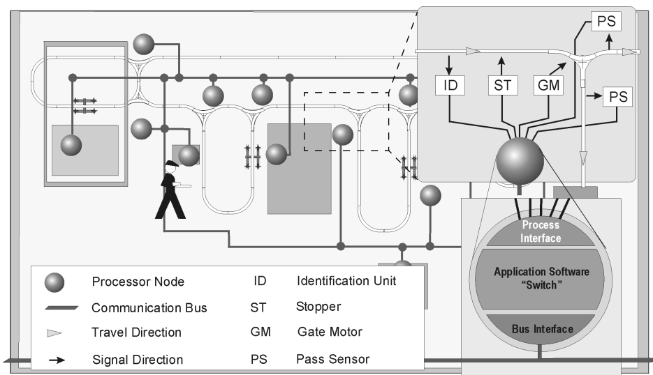
Figure 1 Schematic overview of a material flow system
